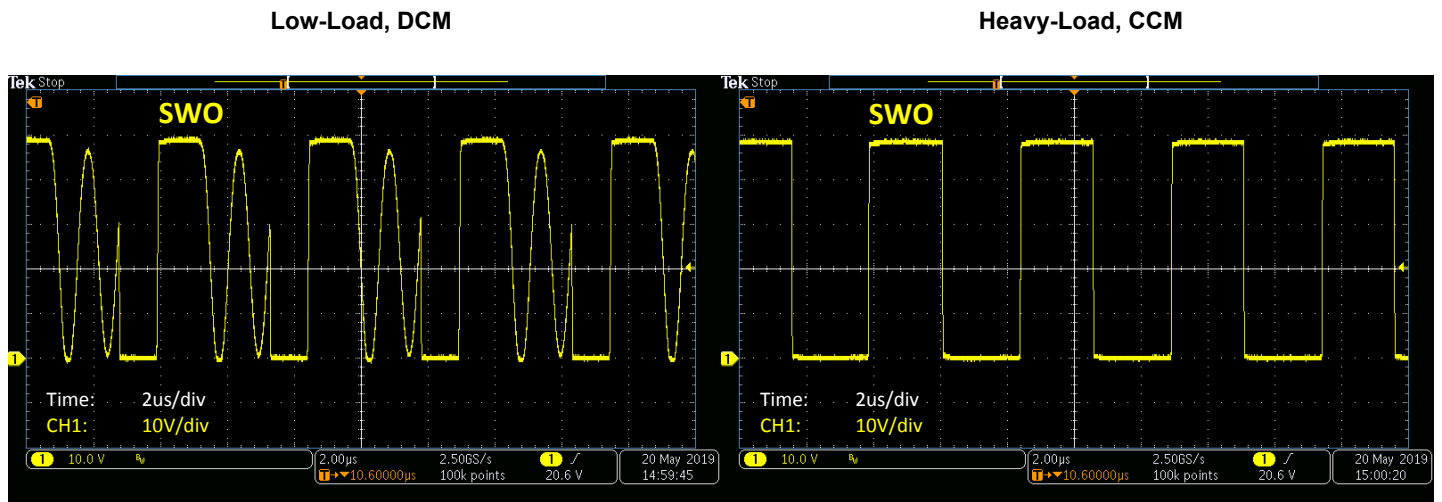
Figure 6.12. Si3404-Buck Non-Isolated, 24 V, Class 3 EVB: SWO Waveform in Discontinuous Current Mode (DCM) at Low Load (Left), and in Continuous Current Mode (CCM) at Heavy Load (Right)
