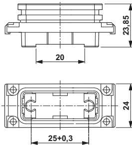
D-SUB panel mounting frame
