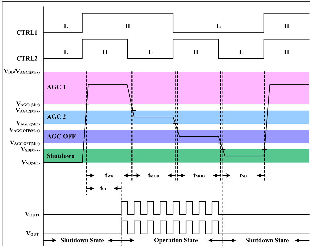
Figure 20 System Timing
