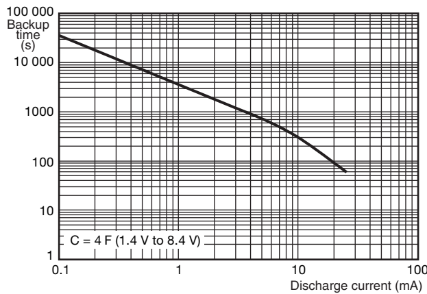
Fig. 18 - Typical Backup Time as a Function of Discharge Current
