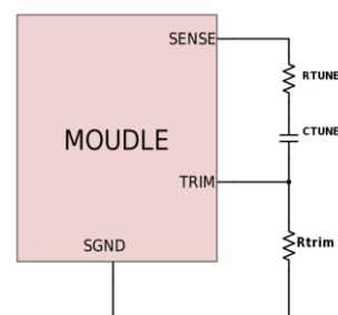
Figure 31. Circuit diagram showing connection of R_{TUNE} and C_{TUNE} to tune the control loop of the module
