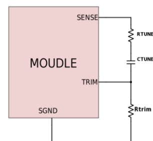
Figure 31. Circuit diagram showing connection of R_{\text{TUNE}} and C_{\text{TUNE}} to tune the control loop of the module
