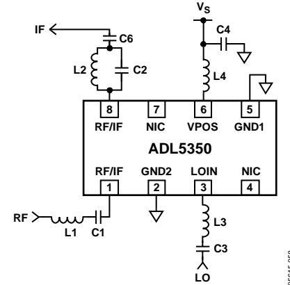
Figure 58. Reference Schematic
