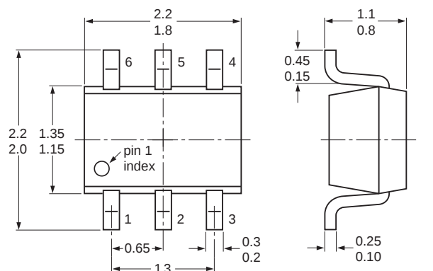
Fig 12. Package outline SOT363 (SC-88)
