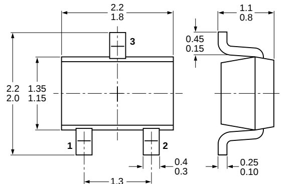
Fig 10. Package outline SOT323 (SC-70)
