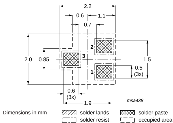
Fig 28. Reflow soldering footprint SOT416
