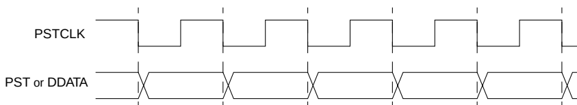
Figure 5-2. PSTCLK Timing
