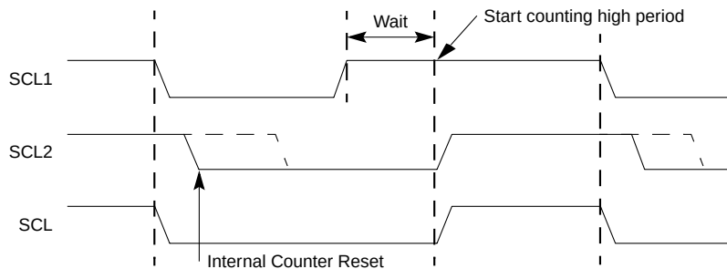
Figure 8-4. Synchronized Clock SCL
