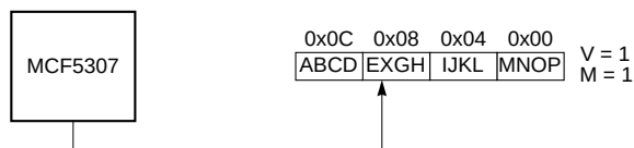
Figure 4-6. Write-Miss in Copyback Mode
