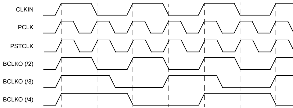
Figure 7-3. CLKIN, PCLK, PSTCLK, and BCLK0 Timing
