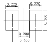
SUGGESTED SOLDER PAD LAYOUT
