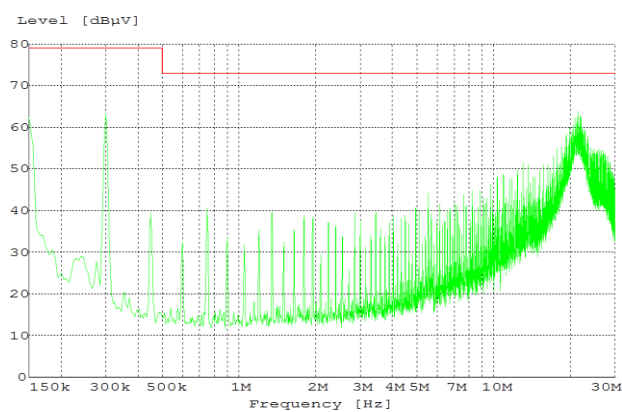
Figure 25. EMC Consideration
