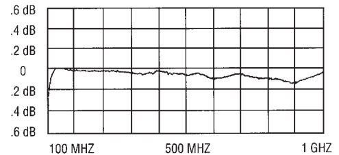
Insertion Loss vs. Frequency for CD17FC621J03, 75 Ω System
