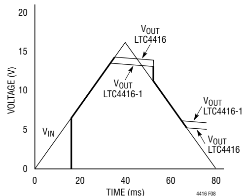
Figure 8. Transient Response of the LTC4416 vs the LTC4416-1 Light Load with a Large Capacitor on V_{\text{OUT}}
