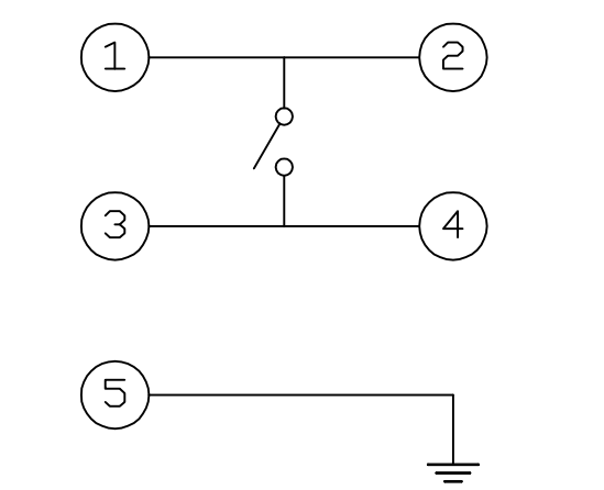
CIRCUIT DIAGRAM
