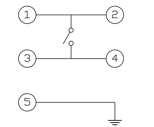
CIRCUIT DIAGRAM
