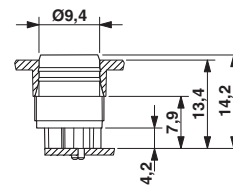
Dimensioned drawing
