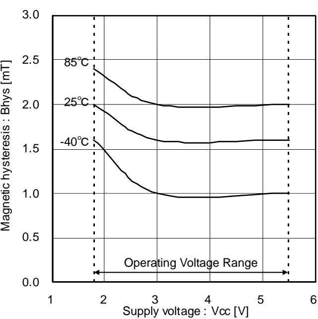
Figure 6. Magnetic hysteresis
