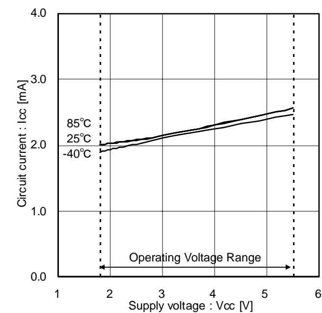
Figure 3. Circuit current 1
