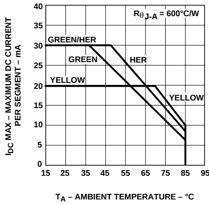
Figure 9. Maximum Allowable DC Current vs. Ambient Temperature. T_{J \text{ MAX}} = 100^\circ\text{C} .
