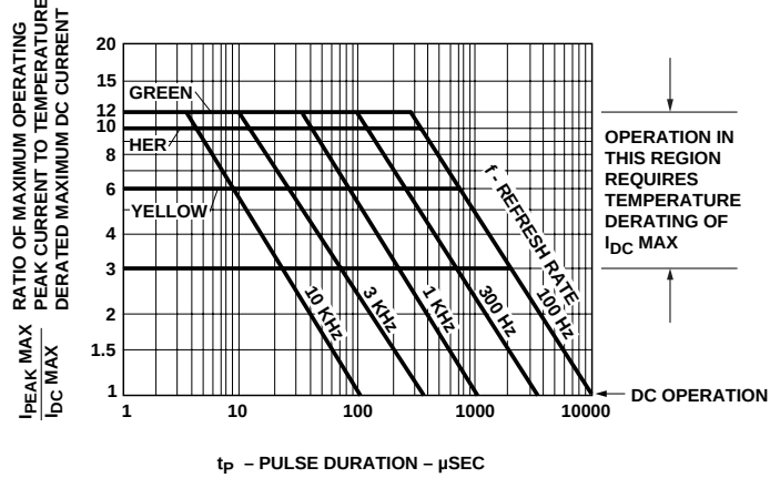
Figure 8. Maximum Tolerable Peak Current vs. Pulse Duration – HER / Yellow / Green.
