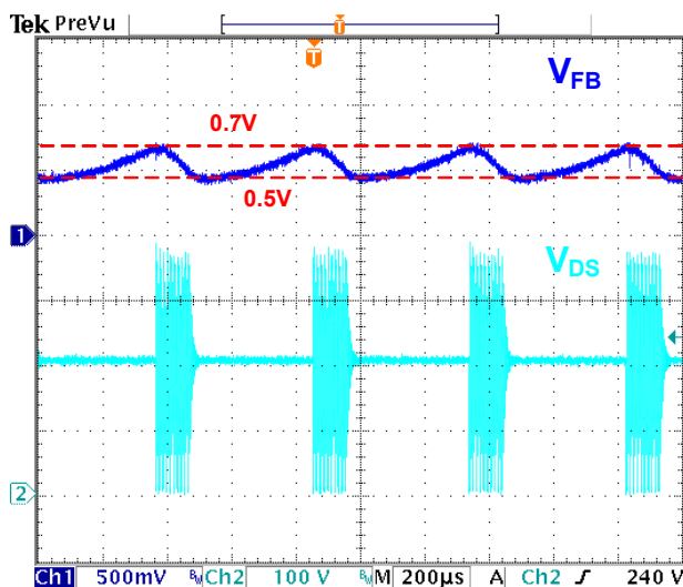
Figure 3: Burst-Mode Operation
