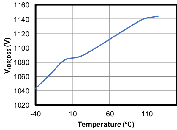
V_{\text{(BR)DSS}} @ I_{\text{Leak}} = 100\mu\text{A} vs. Temperature
