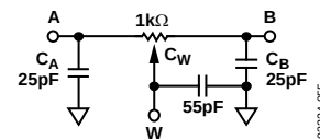
Figure 52. Circuit Simulation Model for RDAC = 1 k \Omega
