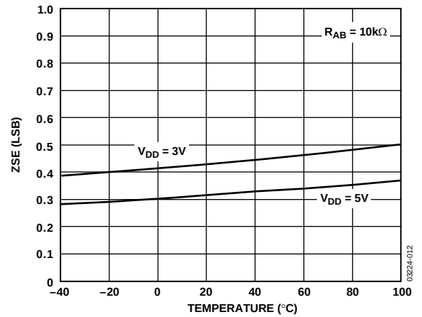
Figure 12. Zero-Scale Error
