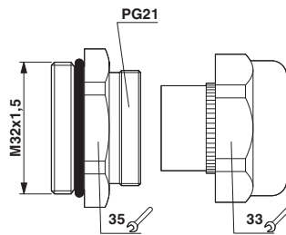
Dimensioned drawing
