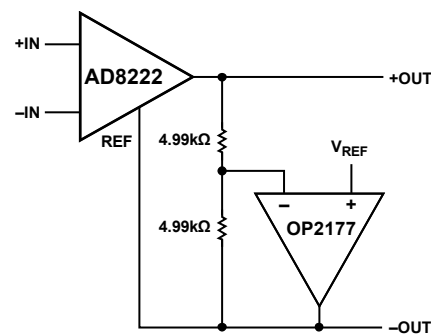
Figure 51. Differential Output Using Op Amp
