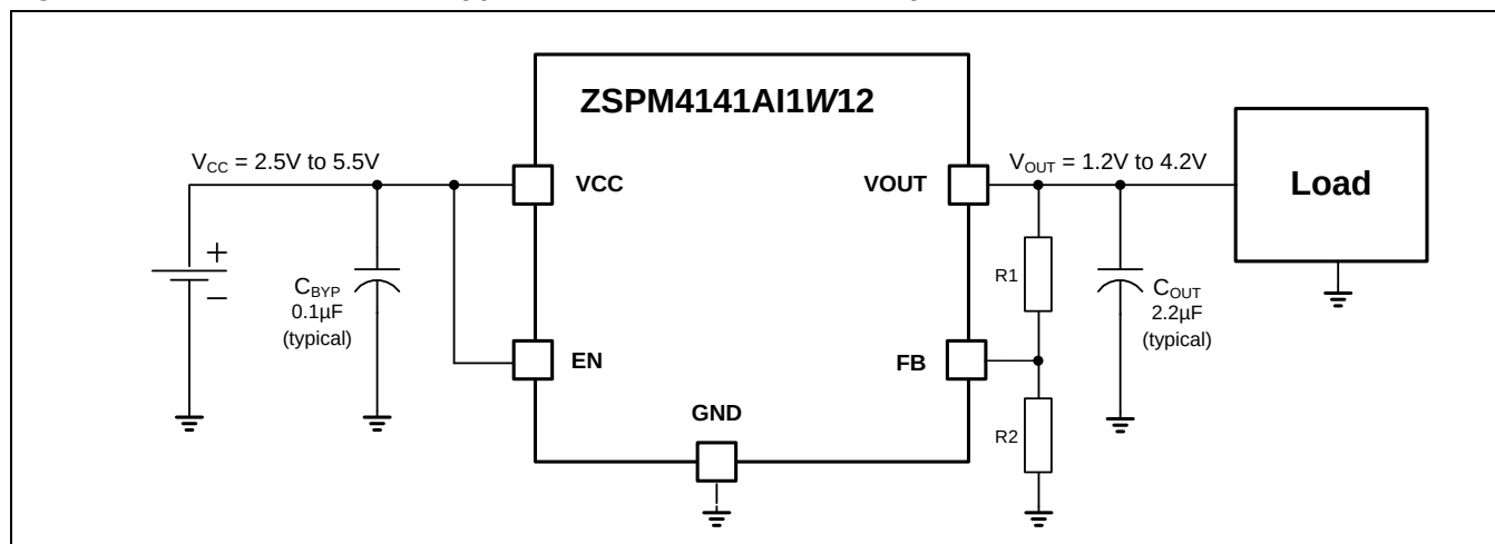
Figure 4.2 ZSPM4141AI1W12 Application Circuit—Variable Output
