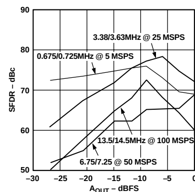
Figure 11. Dual-Tone SFDR vs. A_{OUT} @ f_{OUT} = f_{CLOCK}/7
