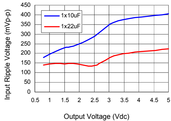
Figure 40. Input ripple voltage for various output voltages with 1 \times 10 \mu\text{F} or 1 \times 22 \mu\text{F} ceramic capacitors at the input (6A load). Input voltage is 12V.
