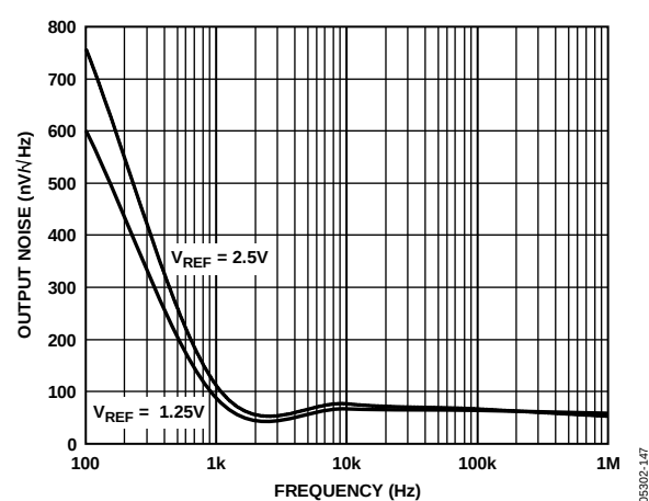
Figure 48. Noise Spectral Density, Internal Reference
