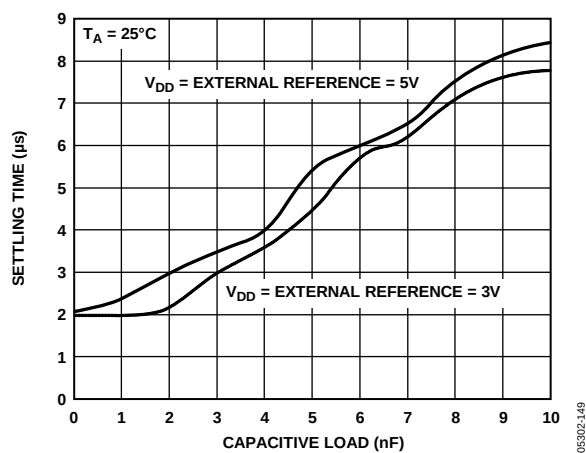
Figure 50. Settling Time vs. Capacitive Load
