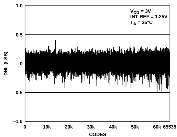
Figure 22. DNL AD5668-1
