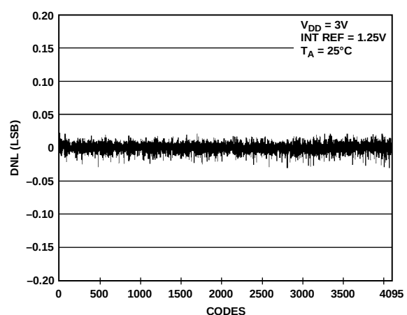
Figure 24. DNL AD5628-1
