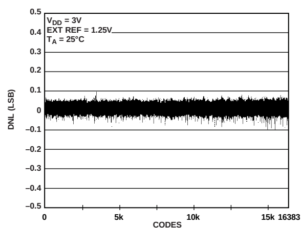
Figure 23. DNL AD5648-1
