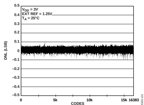
Figure 23. DNL AD5648-1
