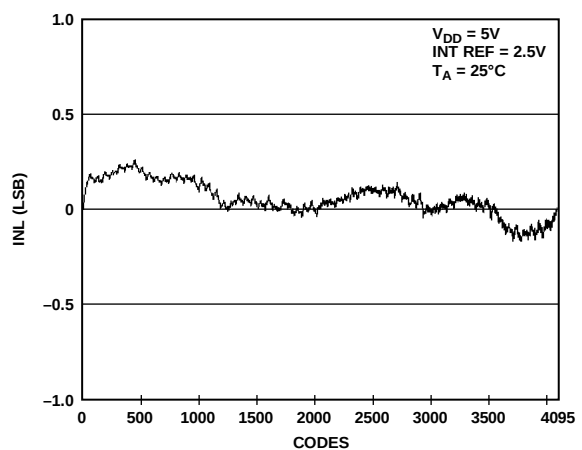
Figure 15. INL AD5628-2
