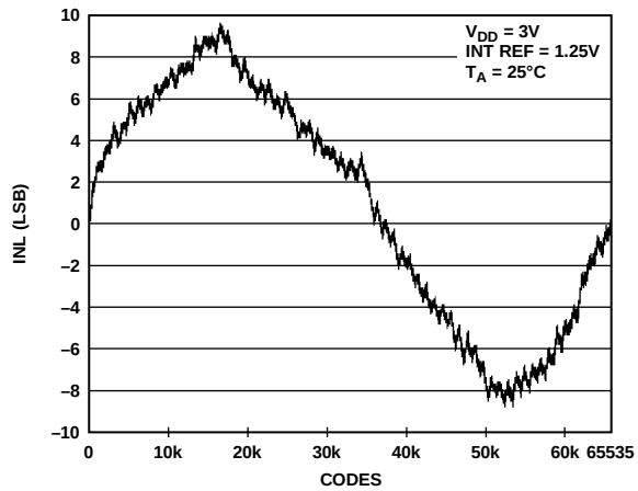
Figure 19. INL AD5668-1
