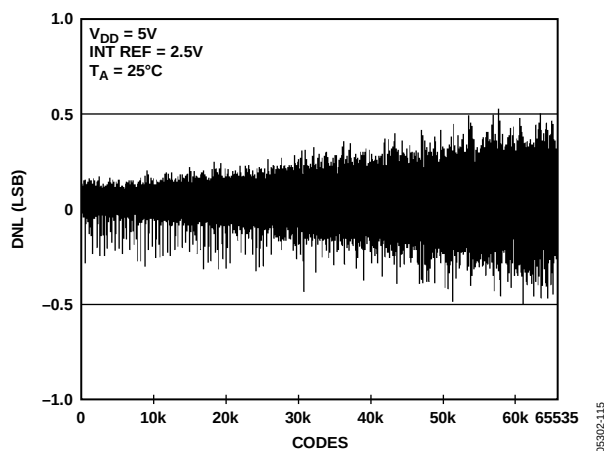
Figure 16. DNL AD5668-2/AD5668-3
