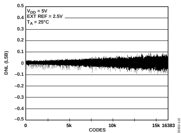
Figure 17. DNL AD5648-2
