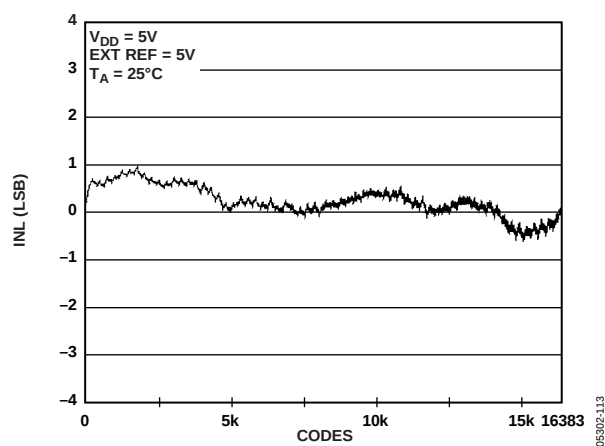
Figure 14. INL AD5648-2
