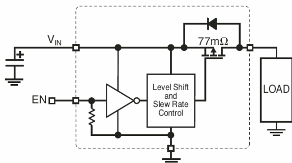
MIC94064 Load Switch Application
