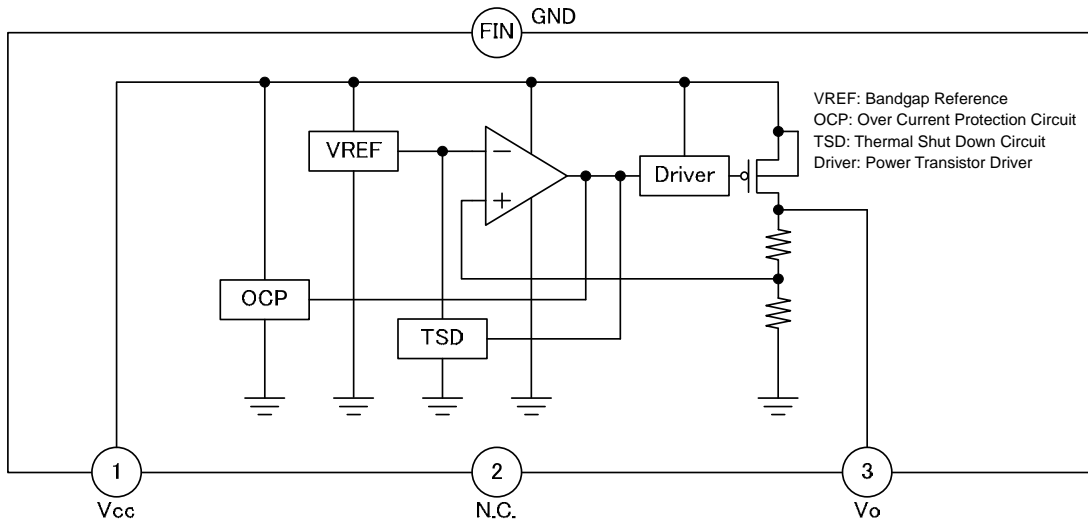
Figure 3. Block Diagram
