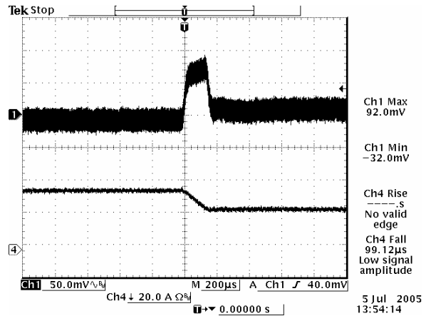
Vout=2.5 V, 75% to 50% Load Transients
