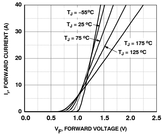
Figure 1. Forward Characteristics
