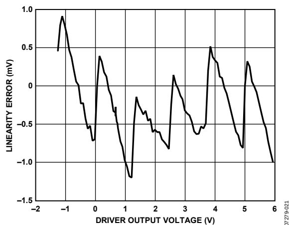
Figure 21. Driver VL Linearity Error
