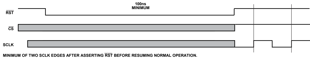
Figure 74. Reset Operation
