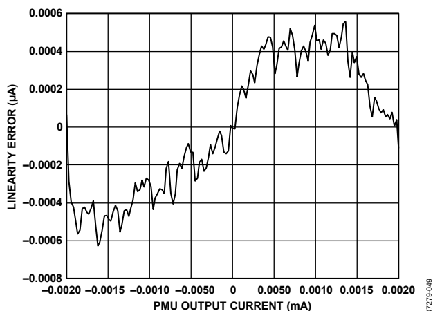
Figure 47. PMU Force Current Range E Linearity
