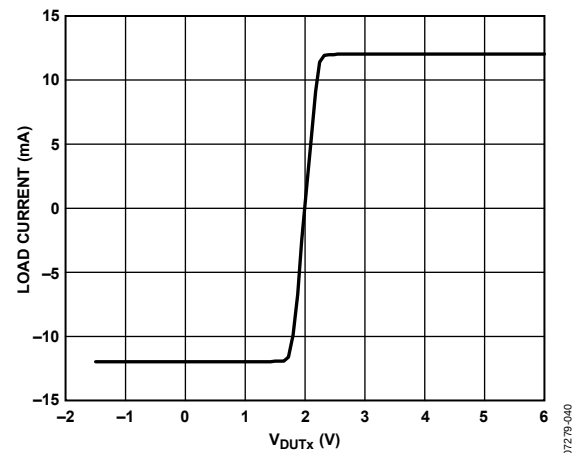
Figure 38. Active Load Commutation Response; V_{COM} = 2.0\text{ V} ; I_{OH} = I_{OL} = 12\text{ mA}
