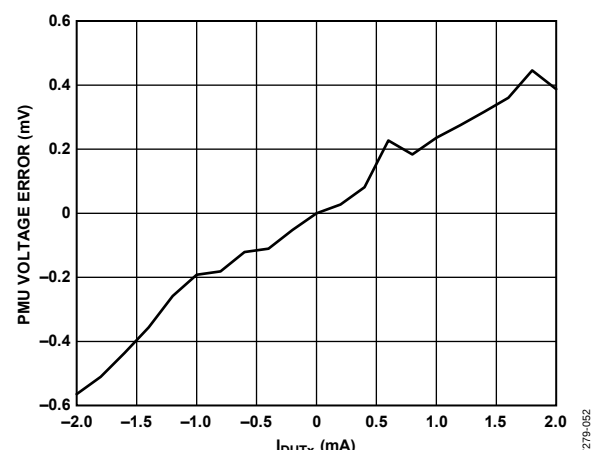
Figure 50. PMU FV Range B Output Voltage Error at 6.75 V vs. Output Current
