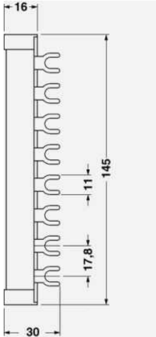
Dimensioned drawing
