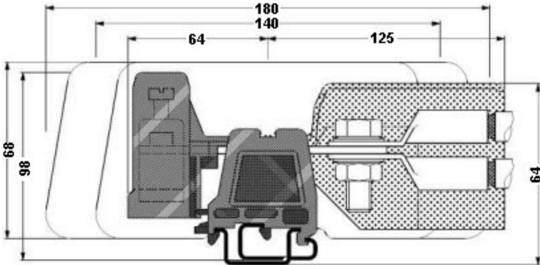
Dimensioned drawing
