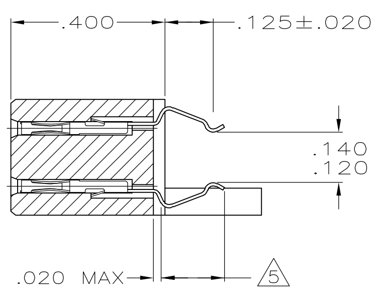
SECTION X-X
