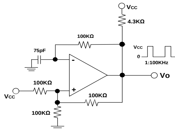
Squarewave Oscillator
