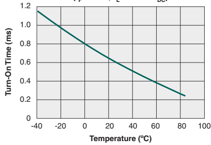
Typical Turn-On Time vs. Temperature ( I_F=5mA, I_L=170mA_{DC} )
