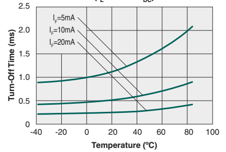
Typical Turn-Off Time vs. Temperature ( I_L=170mA_{DC} )
