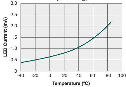
Typical I_F for Switch Dropout vs. Temperature ( I_L=170mA_{DC} )
