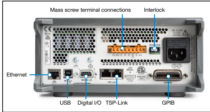
Model 2461 rear panel connections are optimized to maintain signal integrity and speed system setup.
