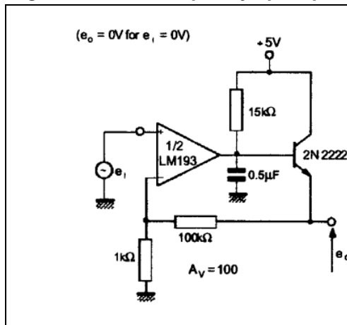
Figure 11. Low-frequency op-amp
