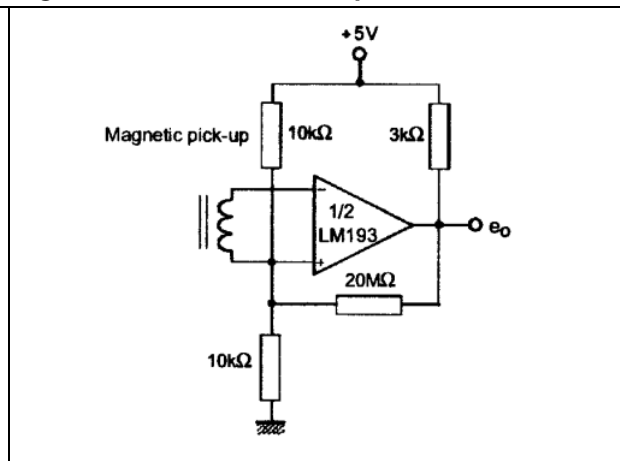
Figure 12. Transducer amplifier
