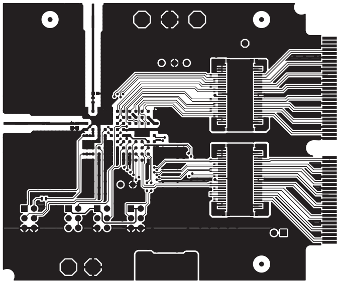
Figure 12. Layer 1 Component Side
