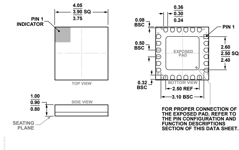
Figure 34. 24-Terminal Ceramic Leadless Chip Carrier [LCC] (E-24-1)
