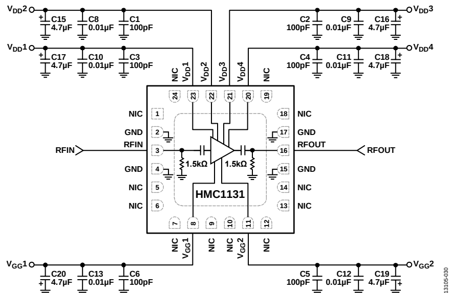
Figure 33. Typical Application Circuit
