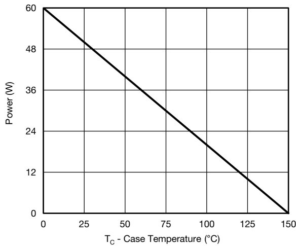
Power, Junction-to-Case
