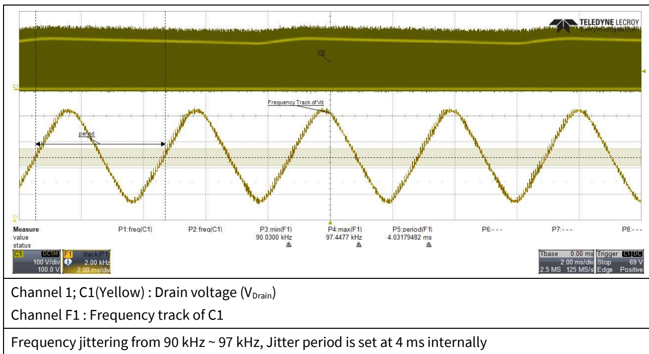
Figure 19 Frequency jittering@ 85 V_{AC} and max. load
