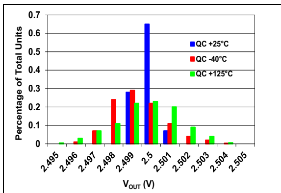
FIGURE 2-20: V_{OUT} at V_{DD\text{MIN}} , V_{DD} = 2.7\text{V} , 800 Units, 2.5V Option, No Load.
